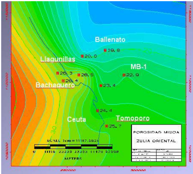
Fig.10 Porosity map based on quartz cement modeling for a medium grained sandstone at the time of the first oil migration
