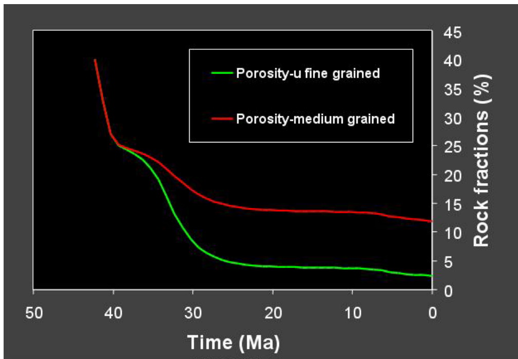
Fig.5 Example of porosity evolution for different grain size lithologies in a given interval
