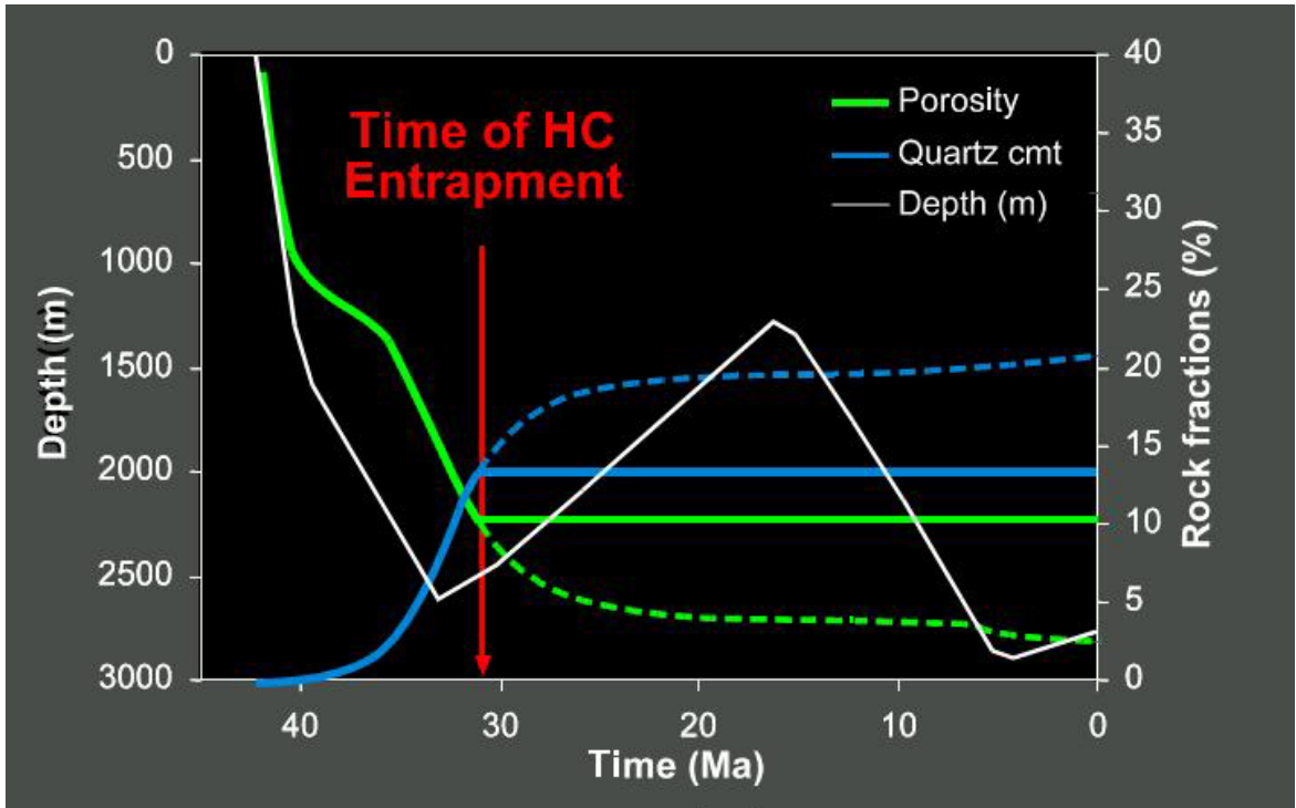
Fig.8 Introduction of hydrocarbon preserves the existing porosity
