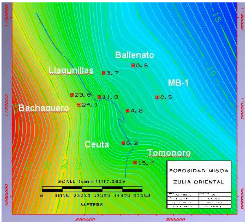
Fig.11 Porosity map based on quartz cement modeling for a medium grained sandstone at the time of the second oil migration
