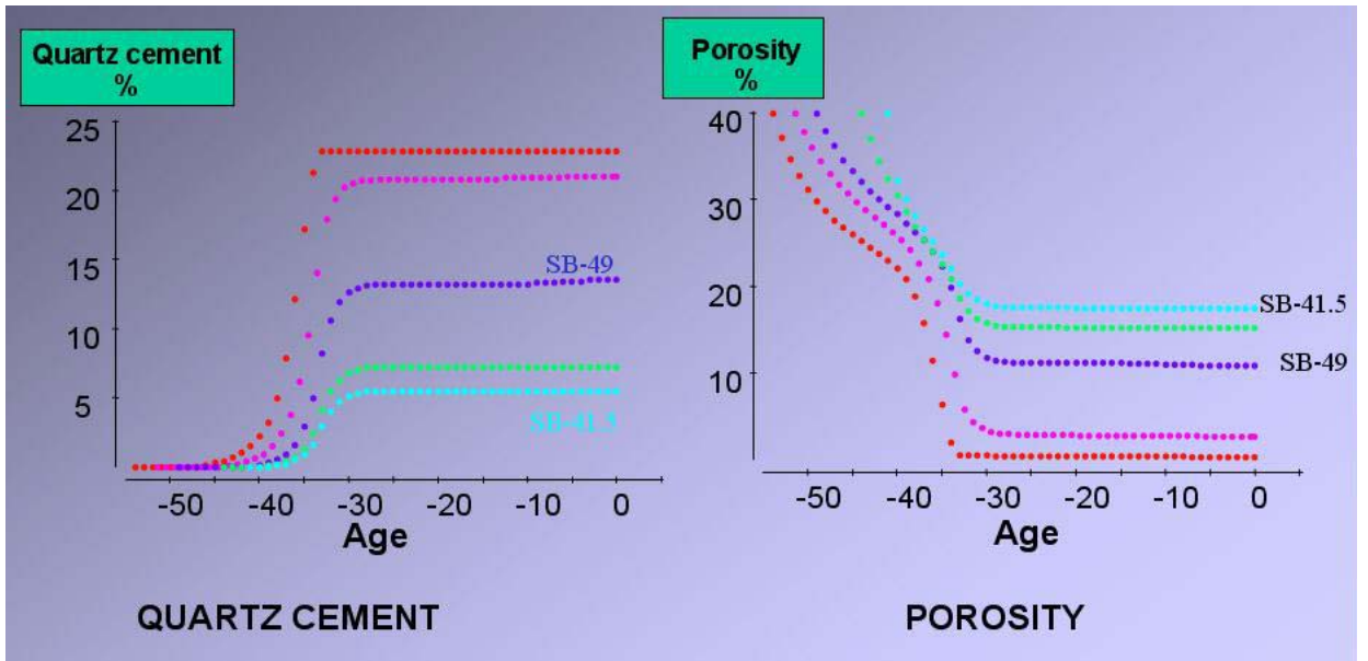
Fig.4 Example of quartz cement and porosity evolution through time for the top of each interval of interest in one well
