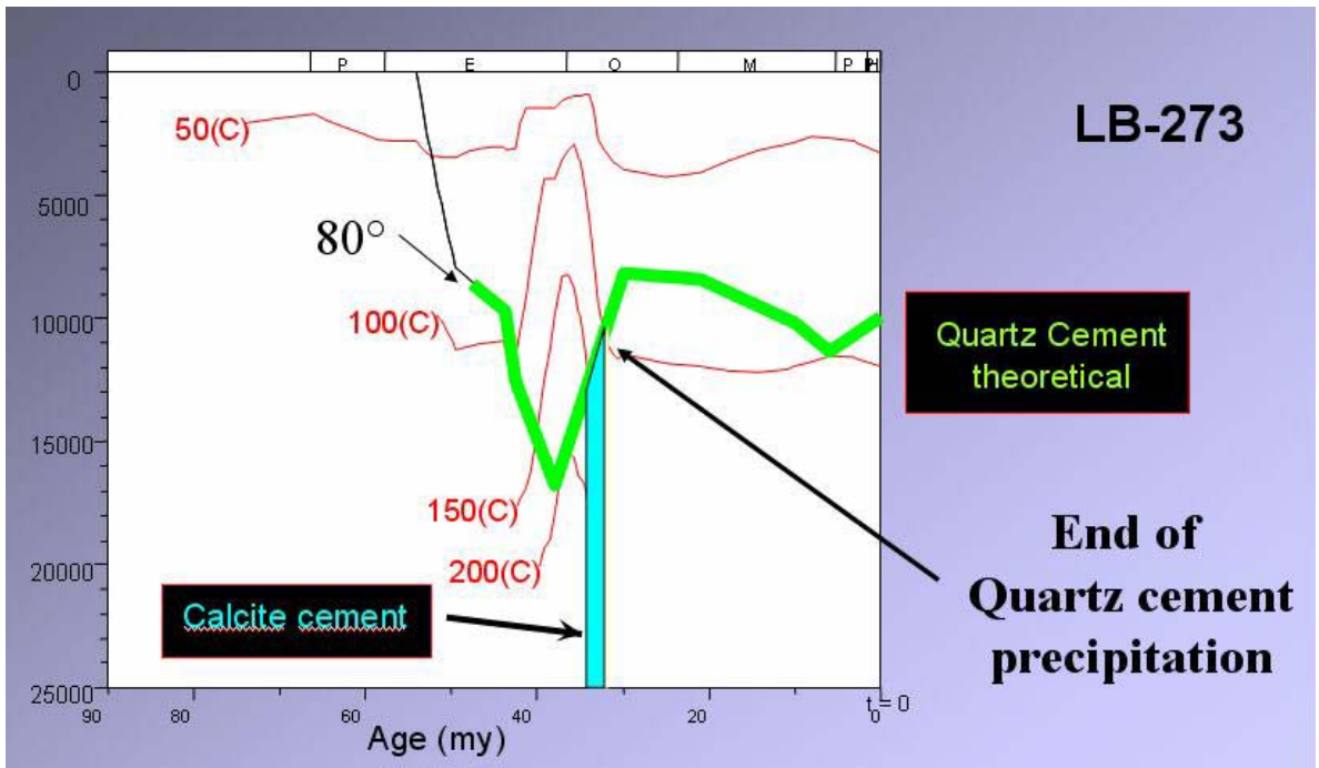
Fig.9 A simple view of the burial and diagenetic history in one well
