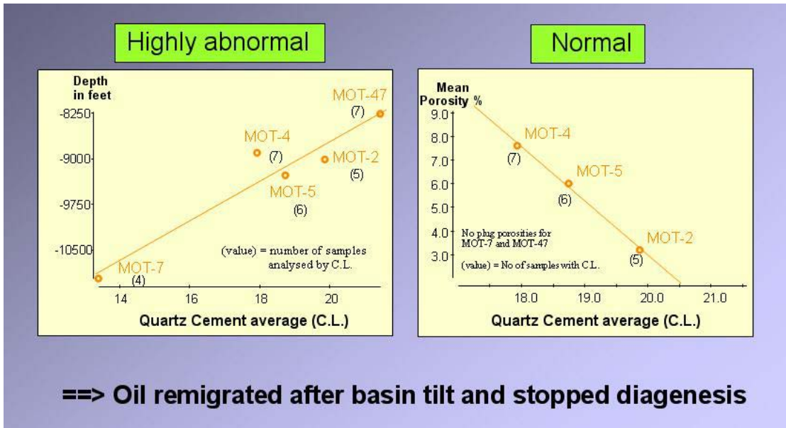
Fig.13 Evidence of basin tilt based on a diagenetic modeling
