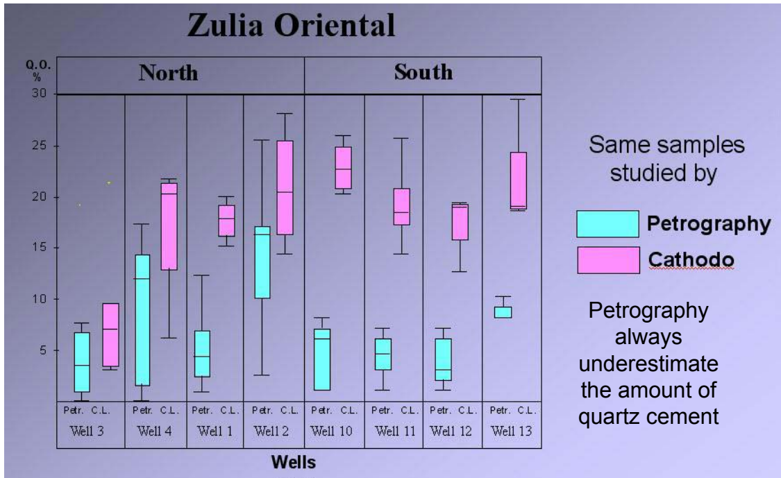
Fig.12 Evidence of the need for cathodoluminescence
