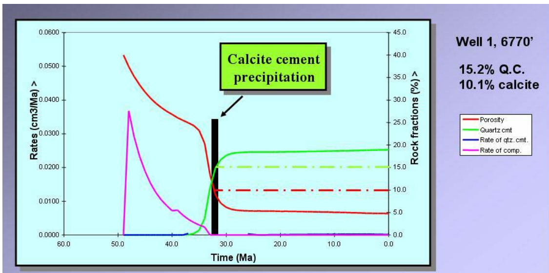
Fig.6 Agreement between amount of calcite cement in and of quartz cement
