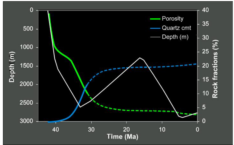
Fig.2 Simulation of quartz cement precipitation and porosity reduction in one well based on the burial history
