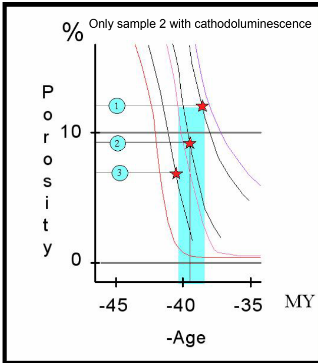
Fig.6 Agreement between amount of calcite cement in and of quartz cement
