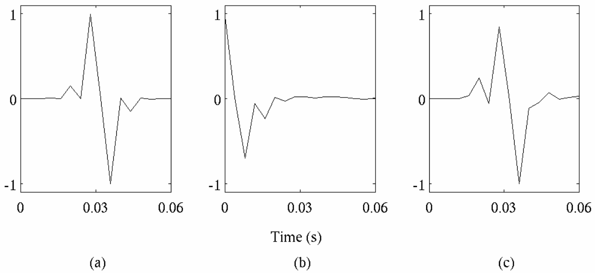
Figure 9. (a) The true 90^\circ phase shifted wavelet. (b) The estimated minimum phase wavelet. (c) The recovered wavelet. Model length p = 4 .
