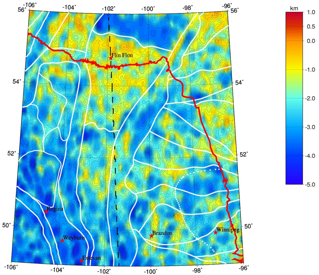
Figure 3. Euler deconvolution result including constraints from logs and seismic data. The red line is the edge of the Canadian Shield. White lines are the interpreted domain boundaries.
