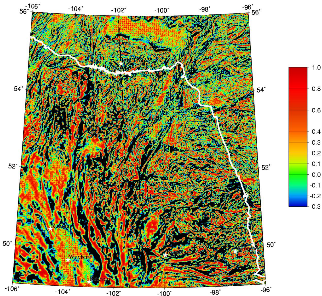
Figure 2. Local Wavenumber image providing high-resolution delineation of magnetic source anomalies. These features are very useful to analysis local and regional structure of basin.
