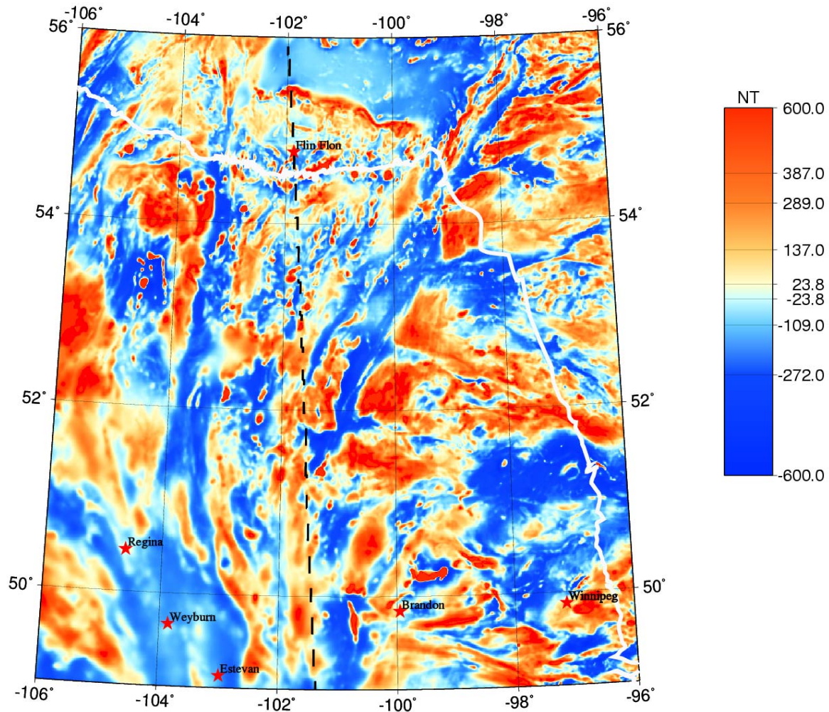
Figure1. Map of aeromagnetic anomaly interpolated and reduced to the pole. White line indicates the edge of the Canadian Shield.
