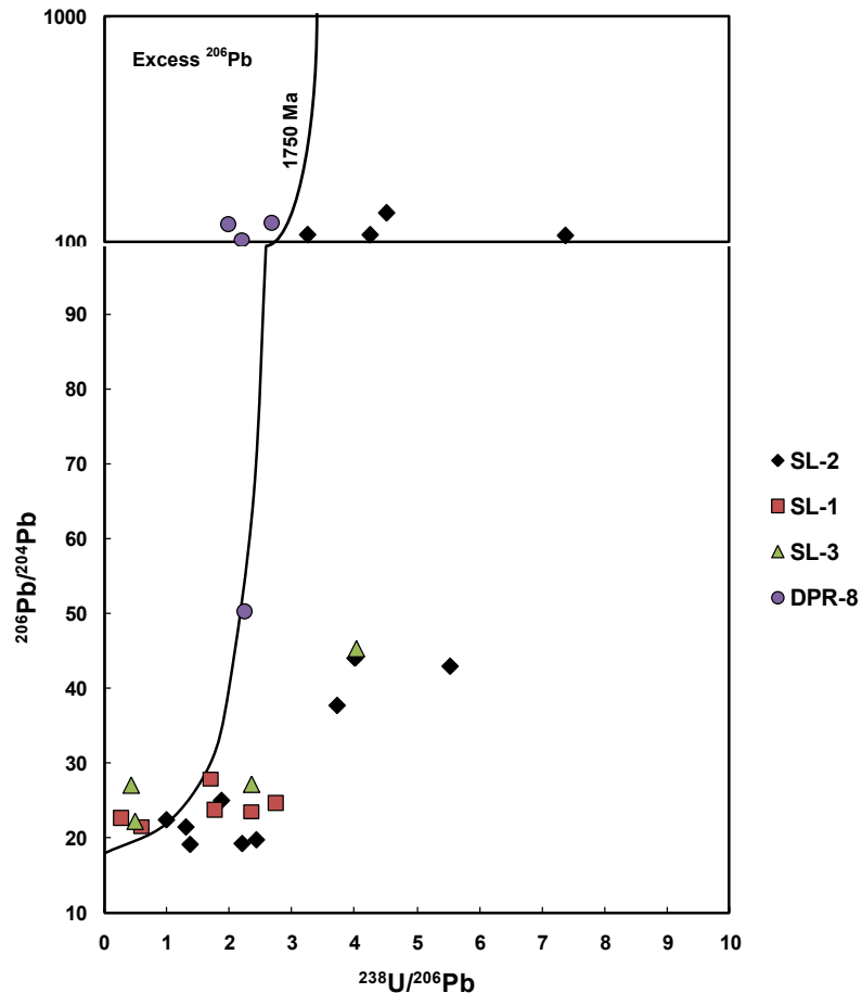
Figure 1: Plot of ^{206}\text{Pb}/^{204}\text{Pb} vs. ^{238}\text{U}/^{206}\text{Pb} for samples extracted by partial-leaching with 2% nitric acid from four drill-holes. The curve is the 1750 Ma U-Pb evolution curve. All samples fall into the area on the left from the curve are interpreted to have ^{206}\text{Pb} contents in excess of the amount of leachable uranium in the sample (Holk et al. 2003).
