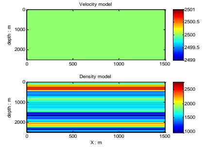
Figure 9. Velocity and density model for a layered earth medium.
