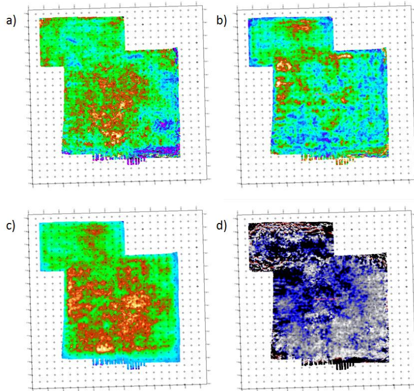
Figure 2: Attribute maps for a) Poisson's ratio, b) Young's modulus, c) P-wave velocity and d) residual moveout. Hot colors represent low values for a) to c) and dark colors represent large residual moveout values for d).
