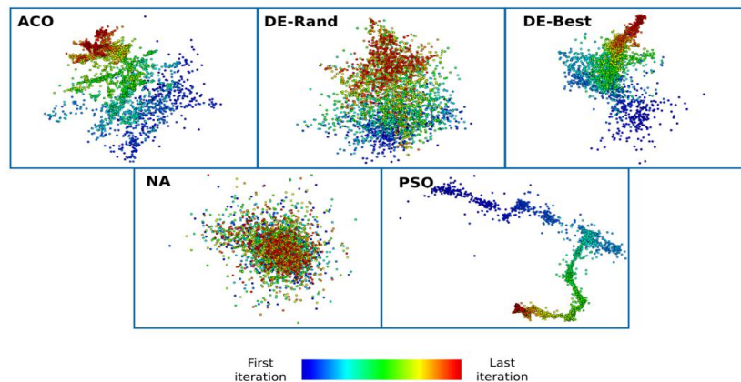
Figure 2 – LSP projection technique to visualize sampling performance of different algorithms
