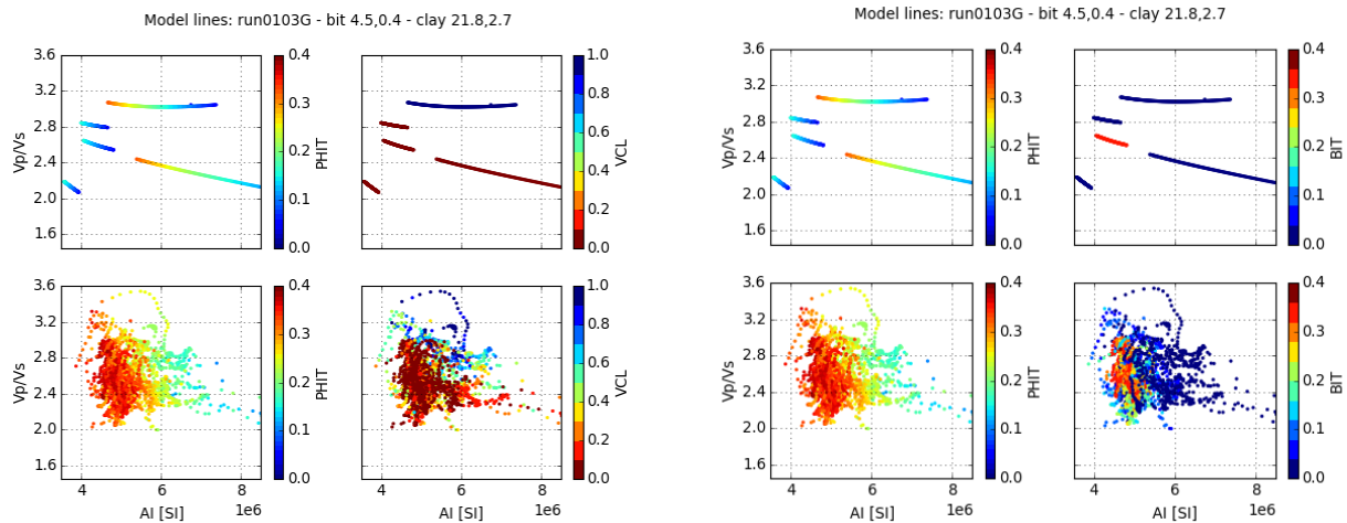
Figure 1 4D rock physics model with sand, clay, bitumen, steam and heated oil trend lines and observed data color coded by porosity and volume of clay (left) and porosity and volume of bitumen (right). Fluid substitution points are shown as shorter trend lines.
