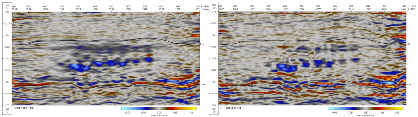
Figure 4 4D inversion results for dAI (left) and dVp/Vs (right) expressed as monitor divided by baseline.
