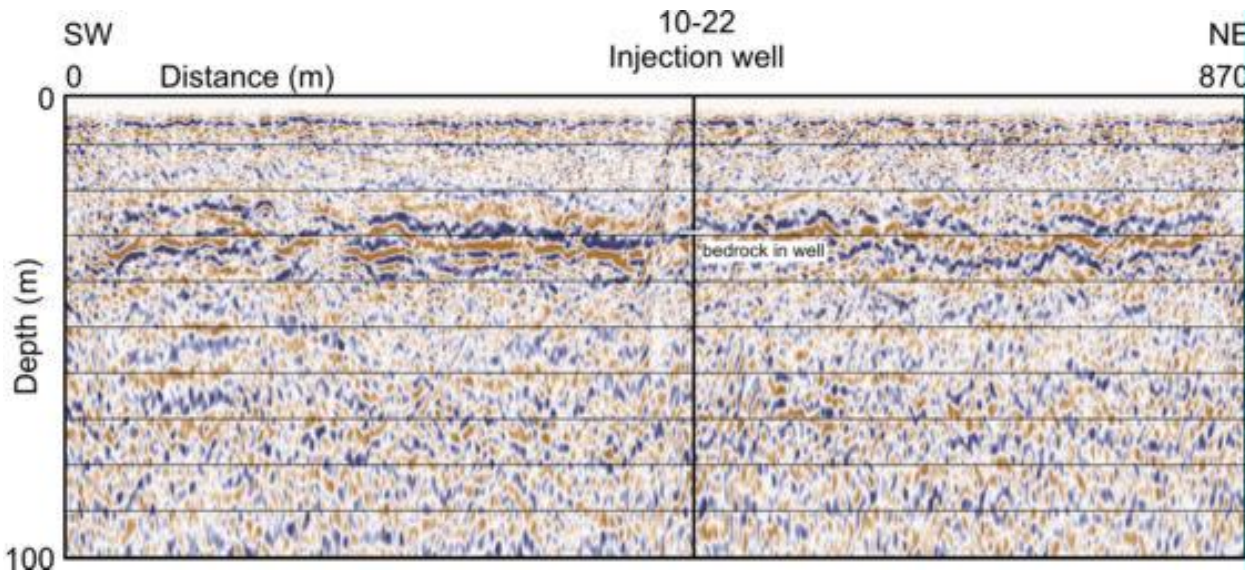
FIG. 2. Migrated towed land streamer array section converted to depth using the velocity model in Figure 1 averaged to a single function. The imaged depth of bedrock compares well to the bedrock depth in the injection well.
