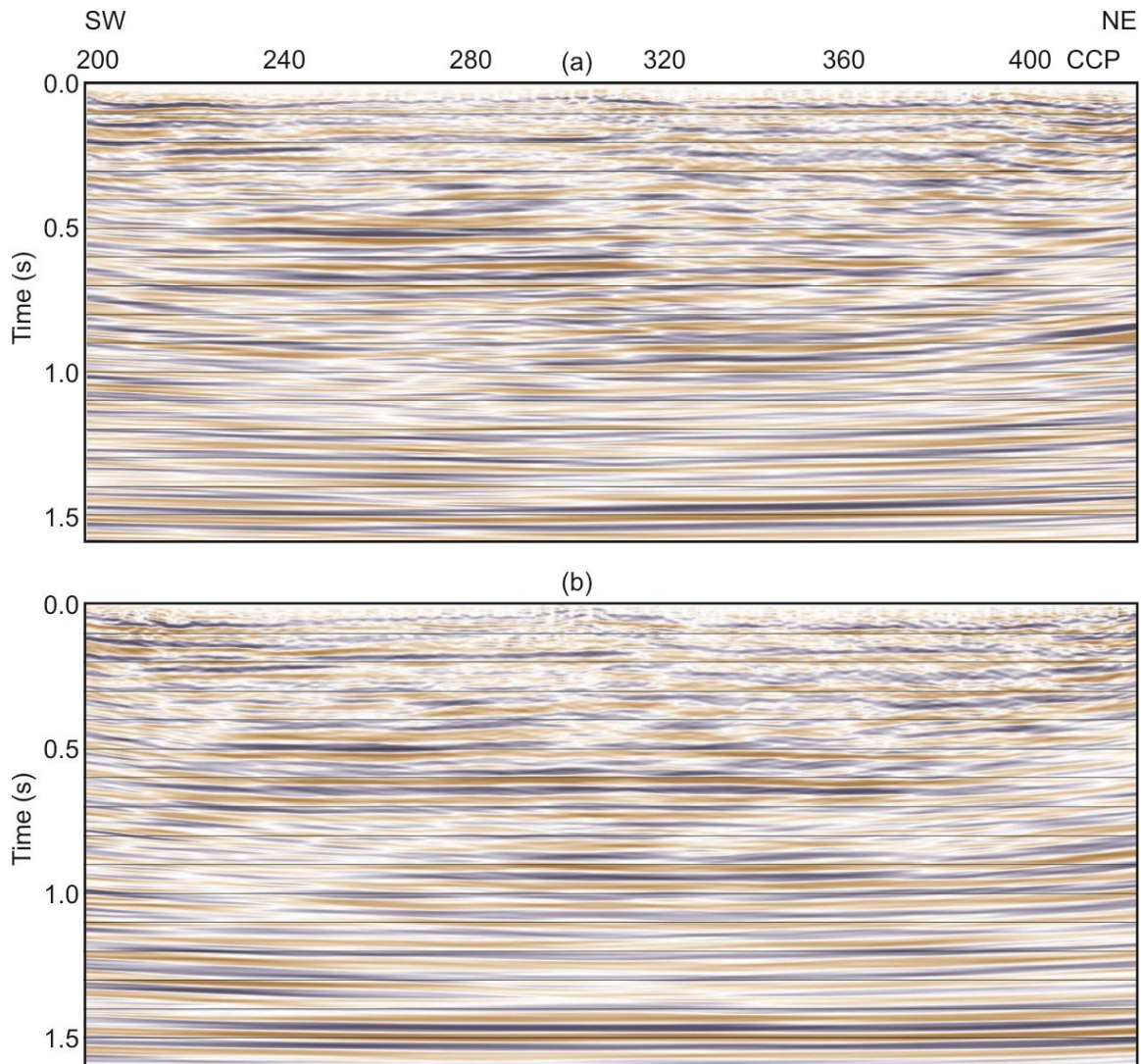
FIG. 3. Migrated CCP stacks of the 2017 PS data with (a) flattening receiver statics, and (b) receiver statics from the 2018 fixed array S-wave survey followed by flattening receiver statics.
