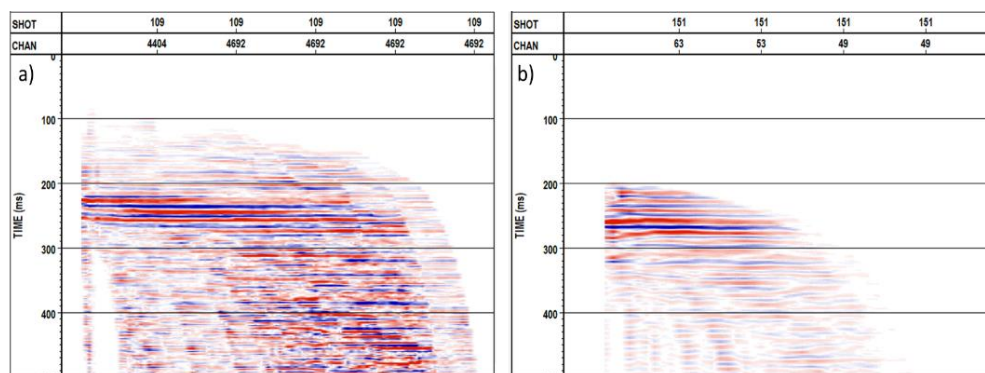
Figure 4 VSP-CDP stacks. a) Straight fibre, b) Geophones.
