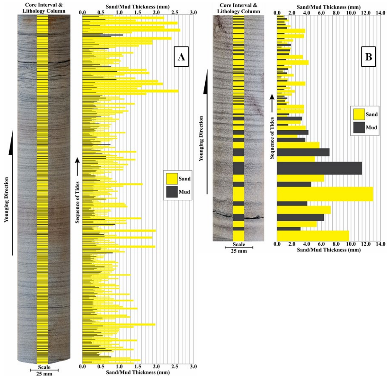
Figure 2. A) Digital photograph of core interval between ~ 810.71 m and ~ 811.02 m with a lithology column showing the sandstone/mudstone laminations. The lamina-thickness plot is to the right. B) Digital photograph of core interval between ~ 1,003.40 m and ~ 1,003.60 m with a lithology column showing the sandstone/mudstone laminations. The lamina-thickness plot is to the right.
