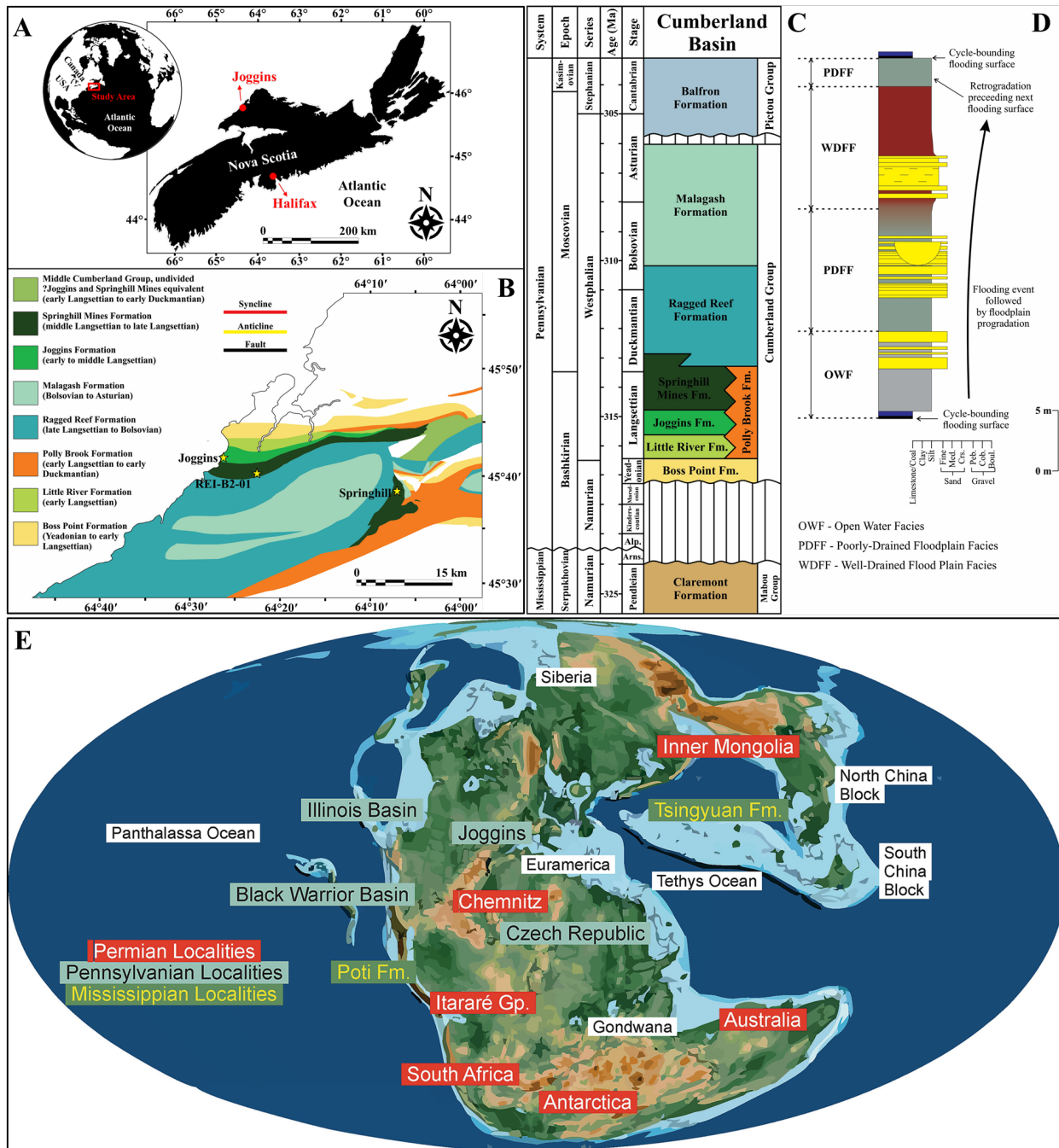
Figure 1. A) Location map showing the study area. B) A closeup view of the study area showing the Cumberland Group geological units and the location of the borehole in relation to Joggins and Springhill. C) The Cumberland Basin stratigraphic framework (modified from Gibling et al. 2008; Gibling et al. 2019). D) A representative measured section of the Joggins Formation (modified from Davies et al. 2005; Gibling et al. 2008; Gibling et al. 2019). E) Permian/Carboniferous paleogeographic map of Pangea showing the main physiographic provinces and the regions containing widespread coal deposits (Gastaldo et al. 2020).
