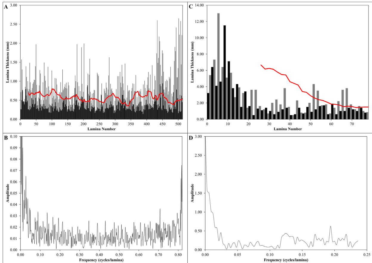
Figure 3. A) Lamina-thickness plot of 516 successive laminae from the interval between ~ 810.71 m and ~ 811.02 m. The grey bars represent the thickness of sandstone and the black bars represent the thickness of mud drapes. The trend line (bold red line) is drawn with a moving average of 14. The younging direction is from left to right. B) The resulting Fourier transformation of the same data. C) Lamina-thickness plot of 79 successive laminae from the interval between ~ 1,003.40 m and ~ 1,003.60 m. The grey bars represent the thickness of sandstone and the black bars represent the thickness of mud drapes. The trend line (bold red line) is drawn with a moving average of 14. The younging direction is from left to right. D) The resulting Fourier transformation of the same data.
